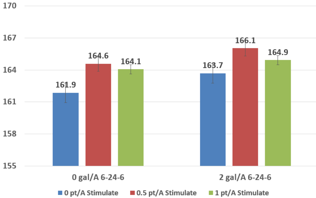
Corn Yield (Bu/A) Results Selected from OSU Hoytville, OH Study +/- 1/2X Fertilizer
