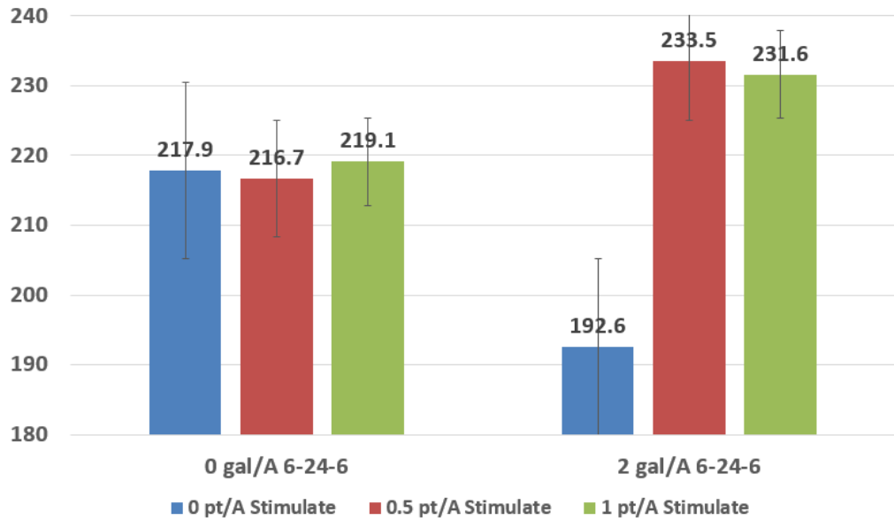
Corn Yield (Bu/A) Results Selected from OSU South Charleston, OH Study +/- 1/2X Fertilizer
